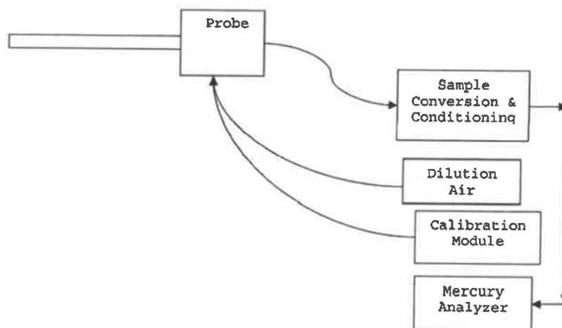
FIGURE A-1. TYPICAL MERCURY CEMS
